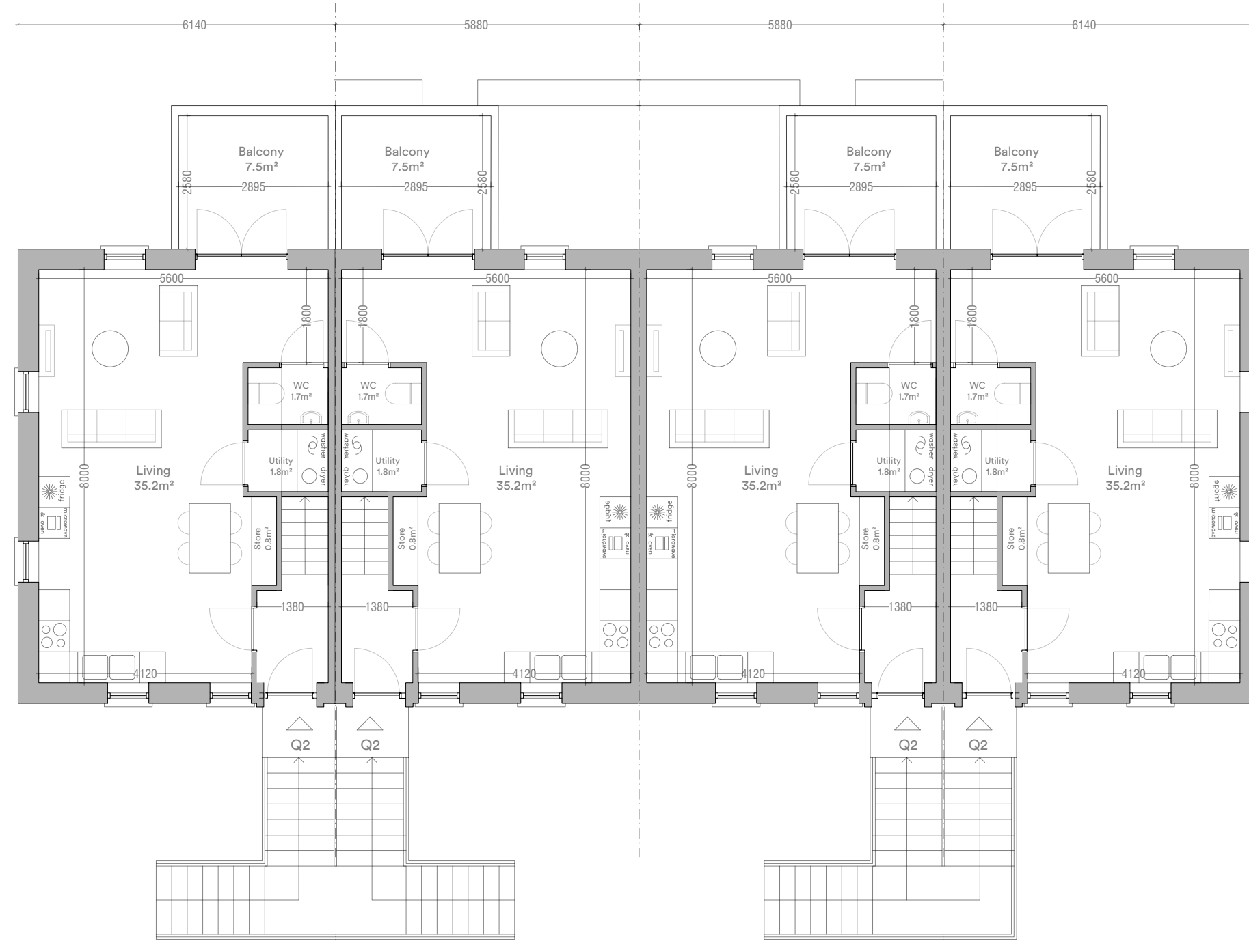
Duplex Block C First Floor
